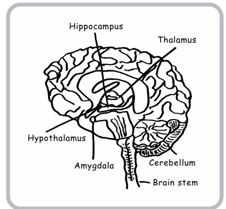
FIGURE 1-3. Limbic system
